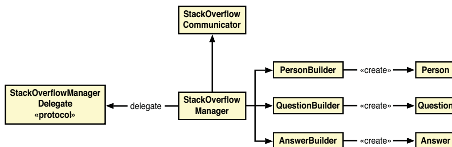
Figure 7.1 Class diagram for the proposed app logic classes.
